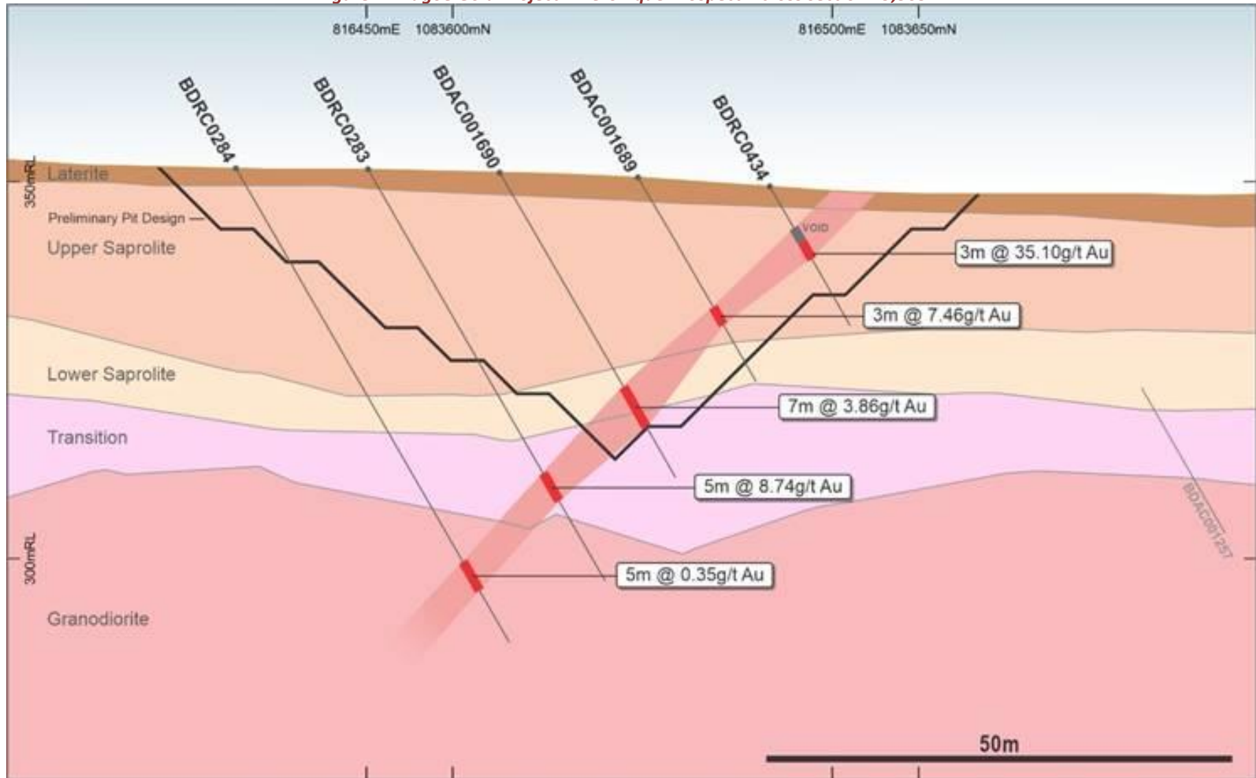
Figure 7: Bagoé Gold Project – Véronique Prospect – cross section 19,565N.
